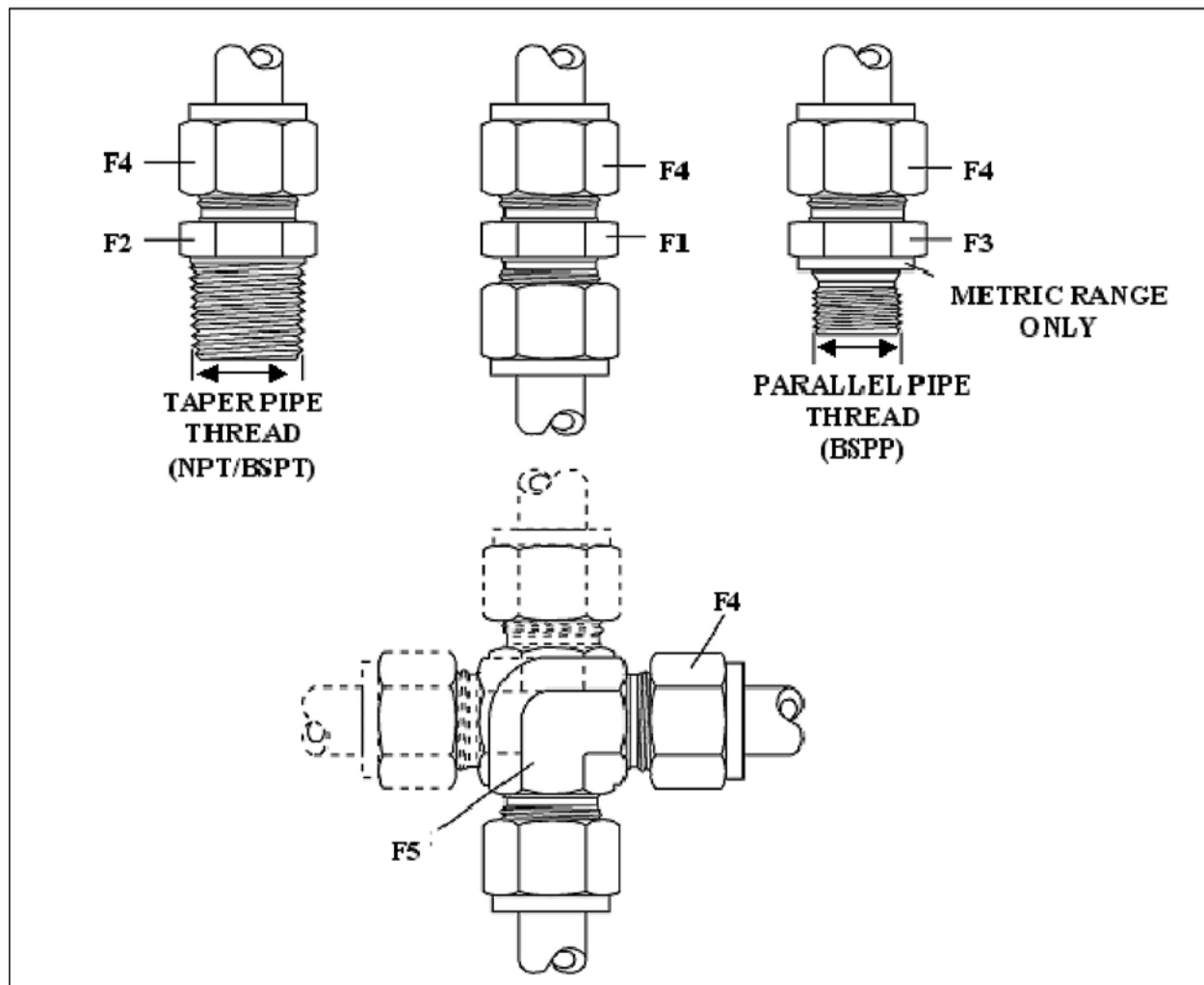
Figure A.3 — Basic dimensions of fittings
