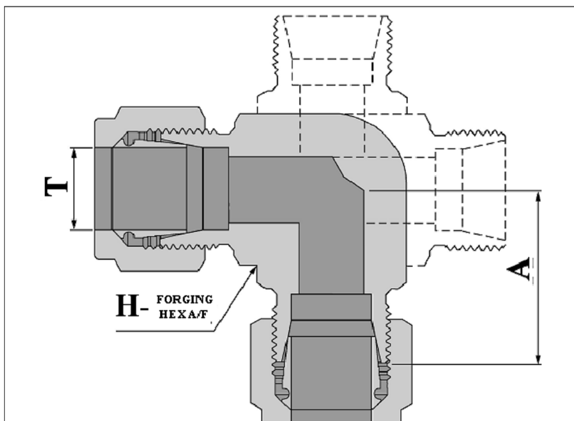
Figure A.4 — End to centre dimensions: equal fittings
