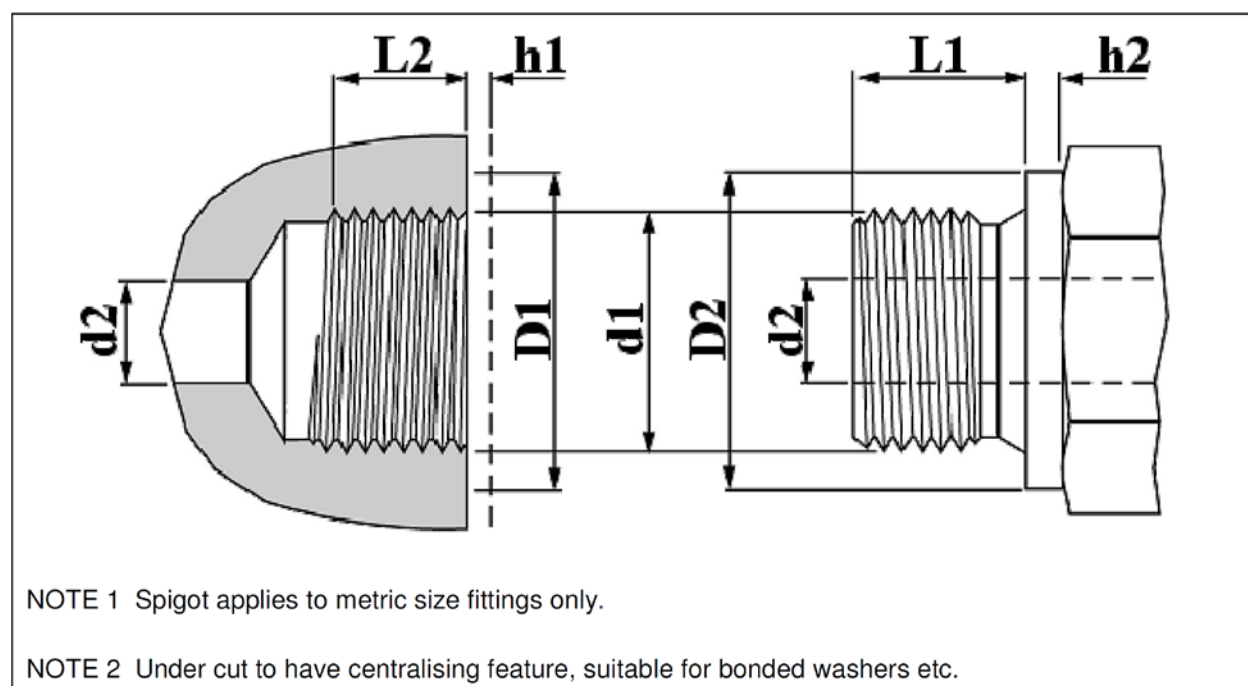
Figure A.7 — BSP parallel connecting threads
