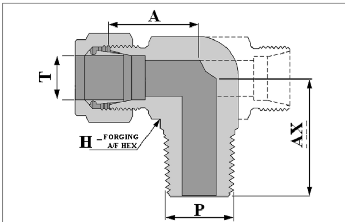
Figure A.5 — End to centre dimensions: male fittings
