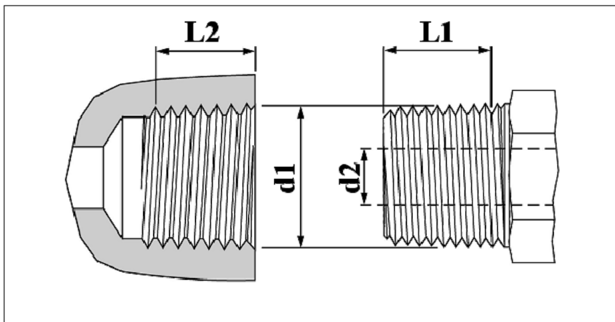
Figure A.8 — BSP taper and NPT taper connecting threads
