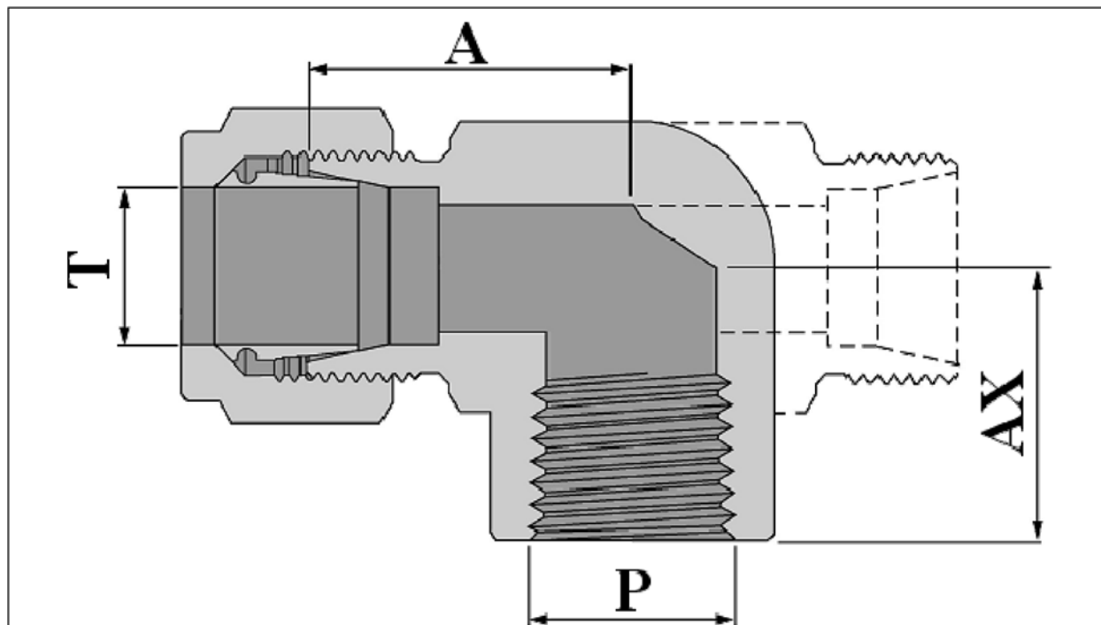
Figure A.6 — End to centre dimensions: female fittings
