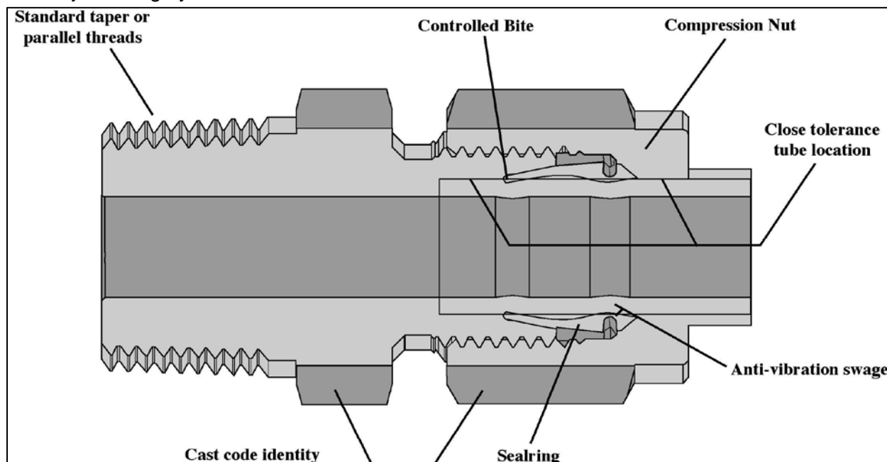
Figure A.1 — Compression fitting: general features
