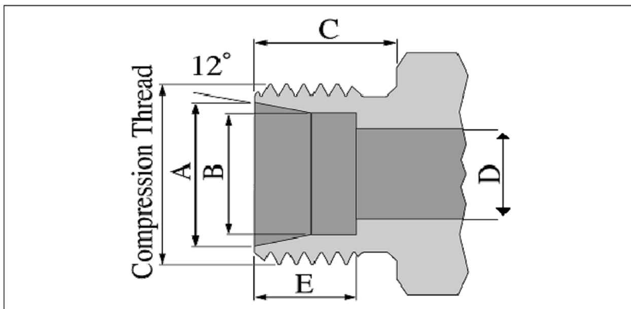
Figure A.2 — Compression end details
